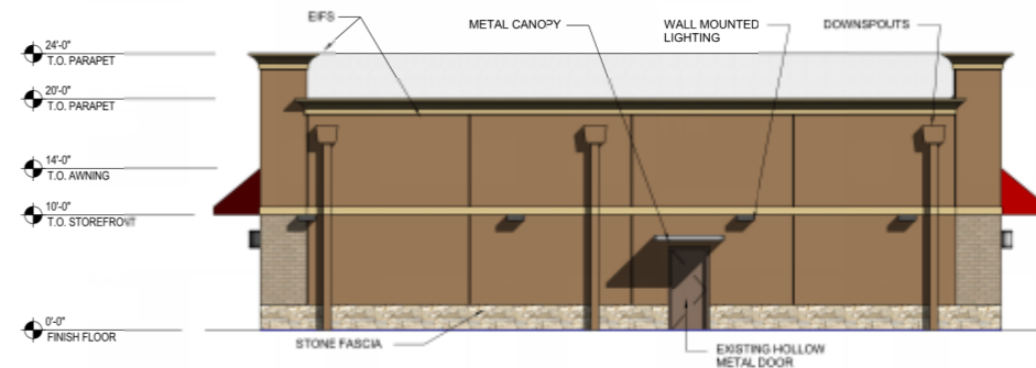
3 SOUTH ELEVATION SCALE: 1:20
